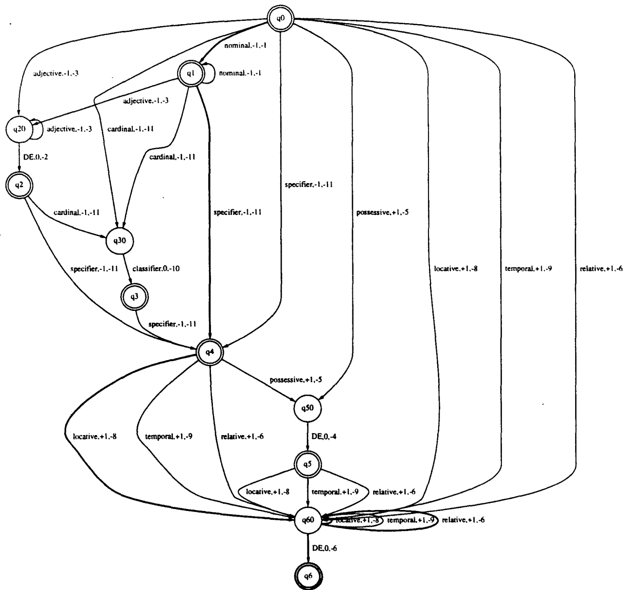
Figure 4: Head transducer for noun phrase dependents
