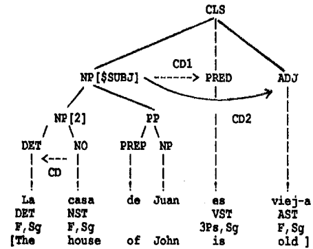
Fig.1: Control Dependences
