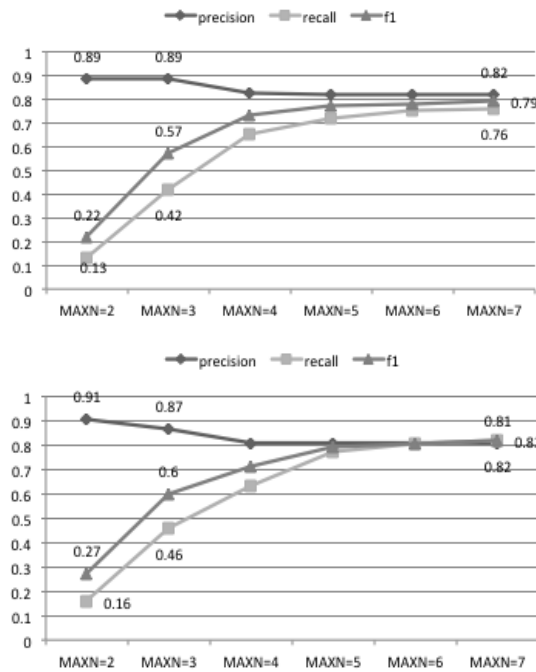
Figure 6. Sentence-level evaluation of the different versions of the system X, with respect to MAXN on the SMT (above) and the RBMT (below) output: Precision, Recall and F1 scores for detecting grammar errors
