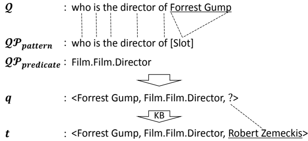
Figure 2: QP -based question translation example
