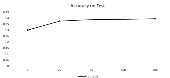
Figure 6: Impacts of beam size on accuracy.
